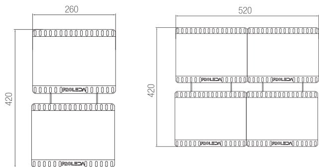
Dimensions (mm)
