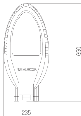
Dimensions (mm)
